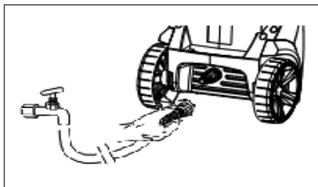
Figure 13 - Attach garden hose to unit (models PW1625 and PW1825)
