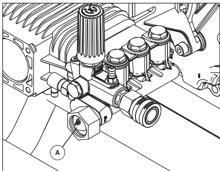
Figure 8 – Inspect Inlet Screen
