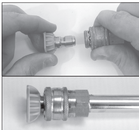
Figure 12 - Inserting quick connect tip
