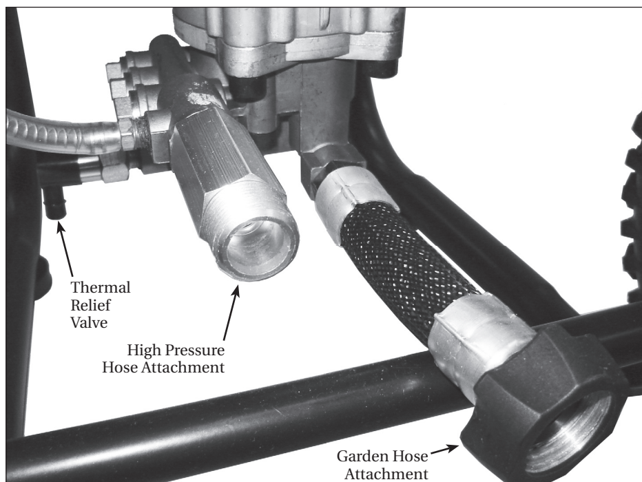
Figure 9 - Pump hook up
