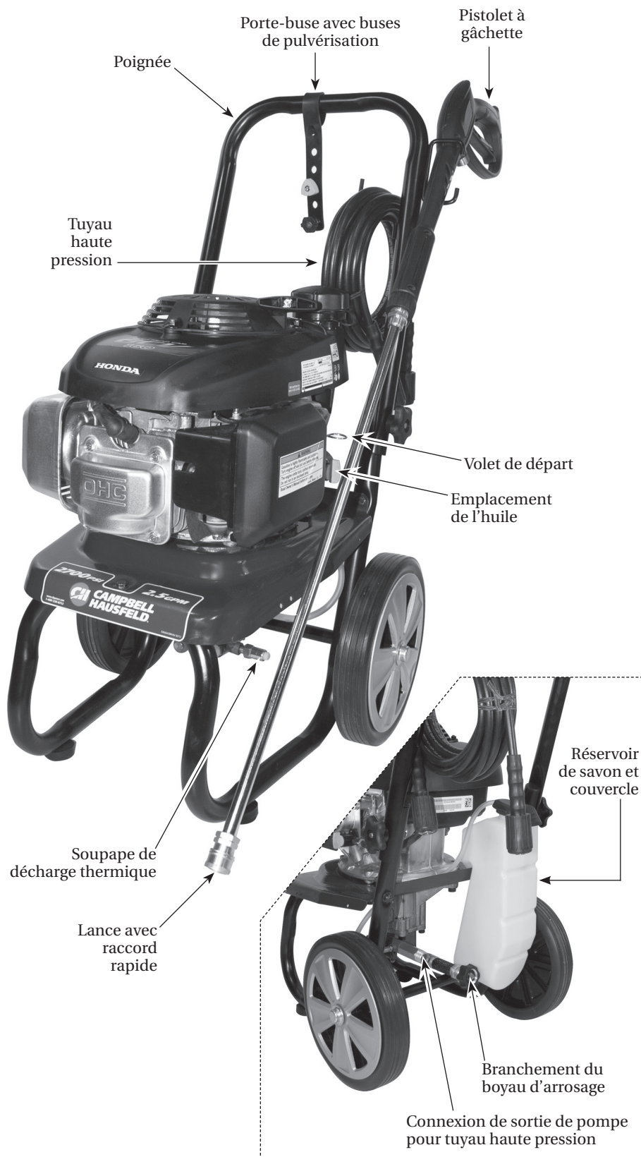
Figure 7 - Components of the Pressure Washer
