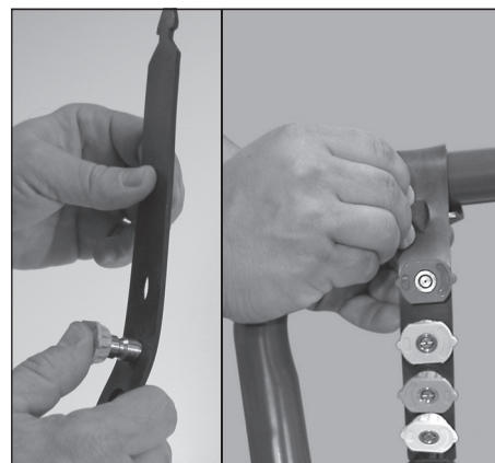
Figure 13 - Insert spray tips into rubber tip holder
