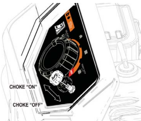
Figure 30 – Choke Knob
