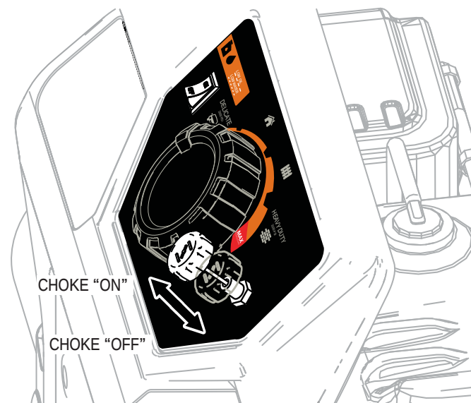
Figure 28 – Choke Knob
