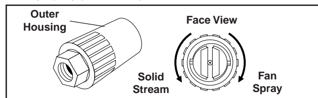
Figure 6 - Nozzle Spray Pattern
